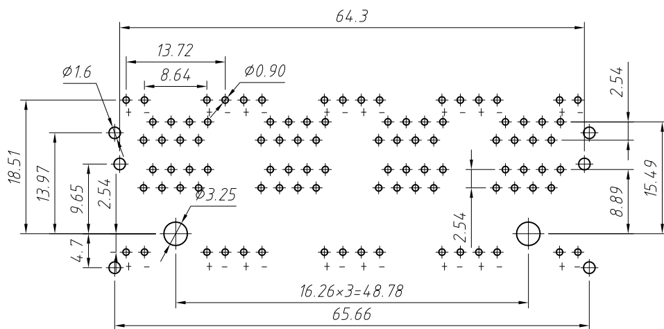
PCB Layout
